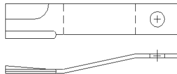
Counter-Clockwise
